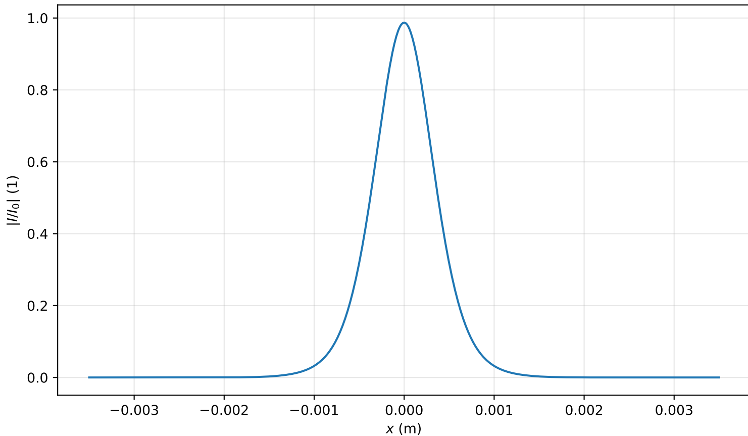
Intensity profile I(x, y = 0, z = 1.831m)/I_0 , P_{in}=0.6P_{cr} , artificial time
